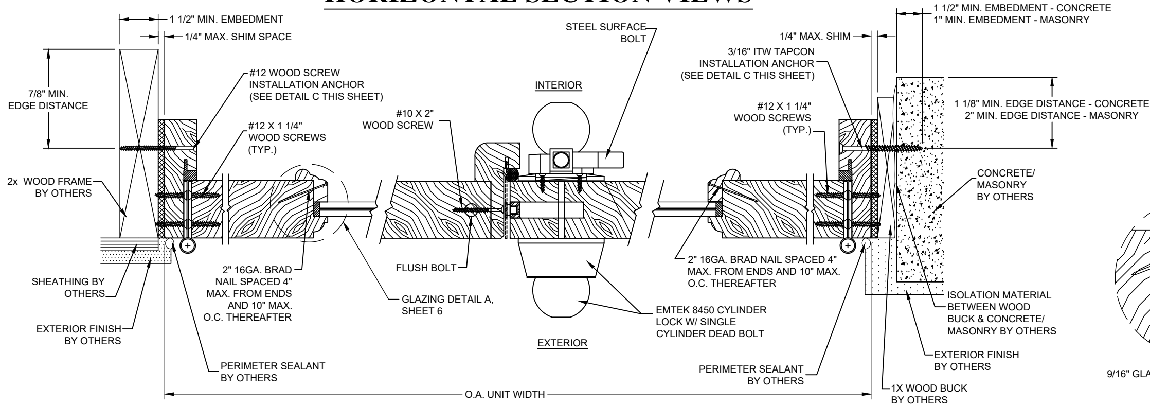
C ) HORIZONTAL SECTION WOOD FRAME SUBSTRATE
