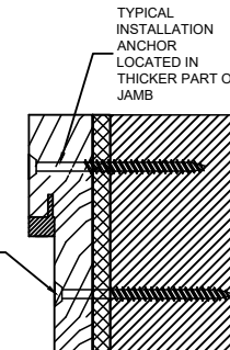
DETAIL B INSTALLATION ANCHOR LOCATION ALTERNATIVES
