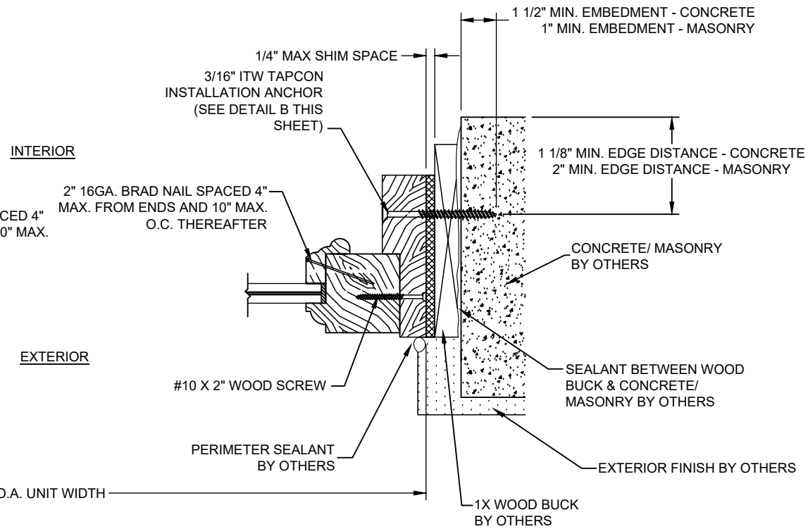
G HORIZONTAL SECTION CONCRETE / MASONRY SUBSTRATE
